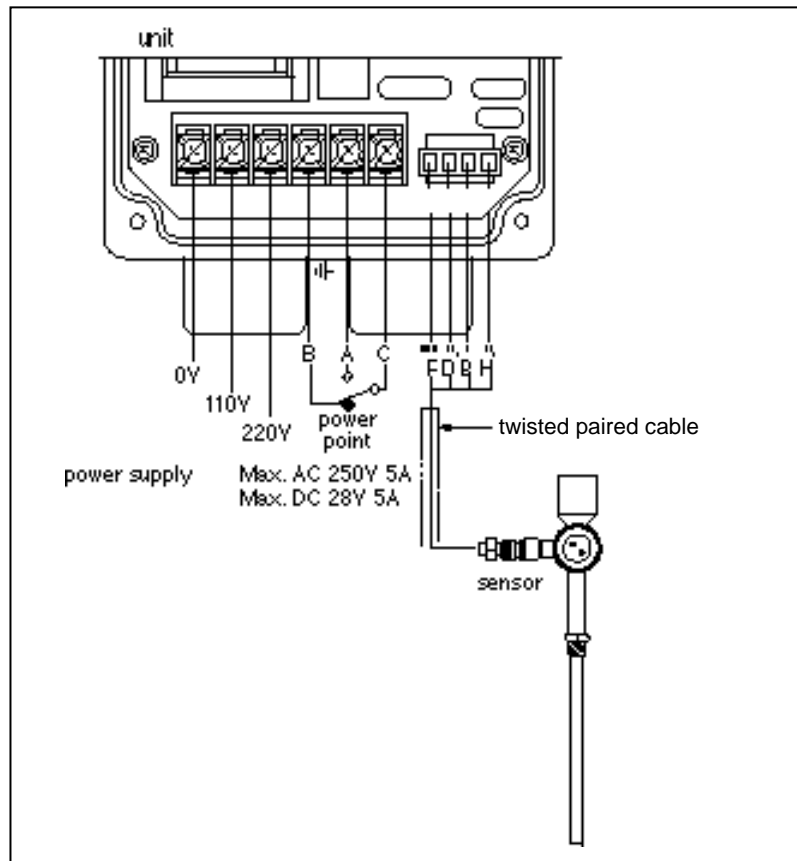
Fig. 2 Schematic diagram for wiring
